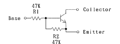
DTC144EU CIRCUIT DIAGRAM
