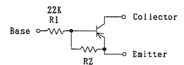
DTA124EU CIRCUIT DIAGRAM
