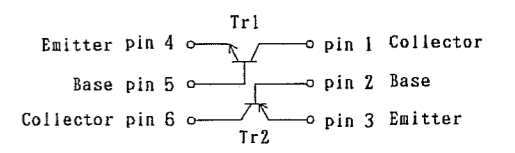
IMZ1 CIRCUIT DIAGRAM
