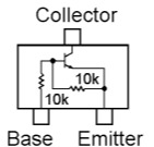
DTC114EU (24) (Q4003, 4006)
