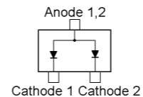
HZM27WA (27A) (D4001) DAP222 (P) (D4002, 4003, 4004, 4005)
