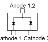
HZM27WA (27A) (D4001) DAP222 (P) (D4002, 4003, 4004, 4005)
