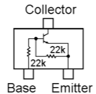
RT1N241M (N2) (Q4011, 4015)
