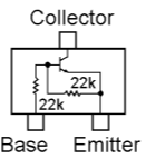
RT1N241M (N2) (Q4011, 4015)
