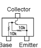
DTC114EU (24) (Q4003, 4006)
